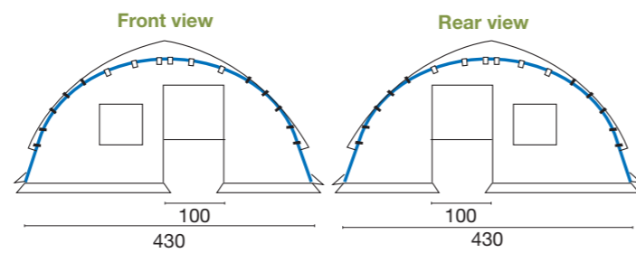
Technical drawing (All measurements in cm)
